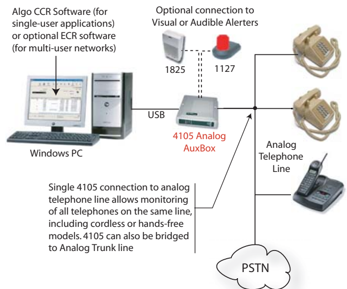
Diagram 1: Connection to Analog Line
