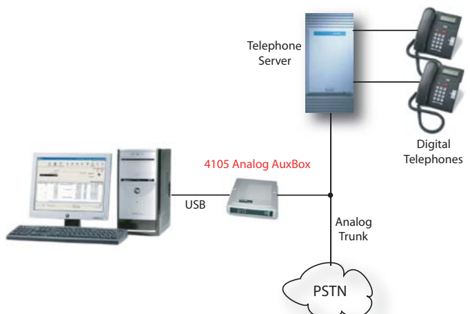
Diagram 2: Connection to Analog Trunk
